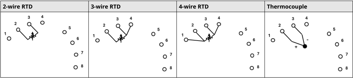
Figure 6: Single Sensor Wiring Diagram
