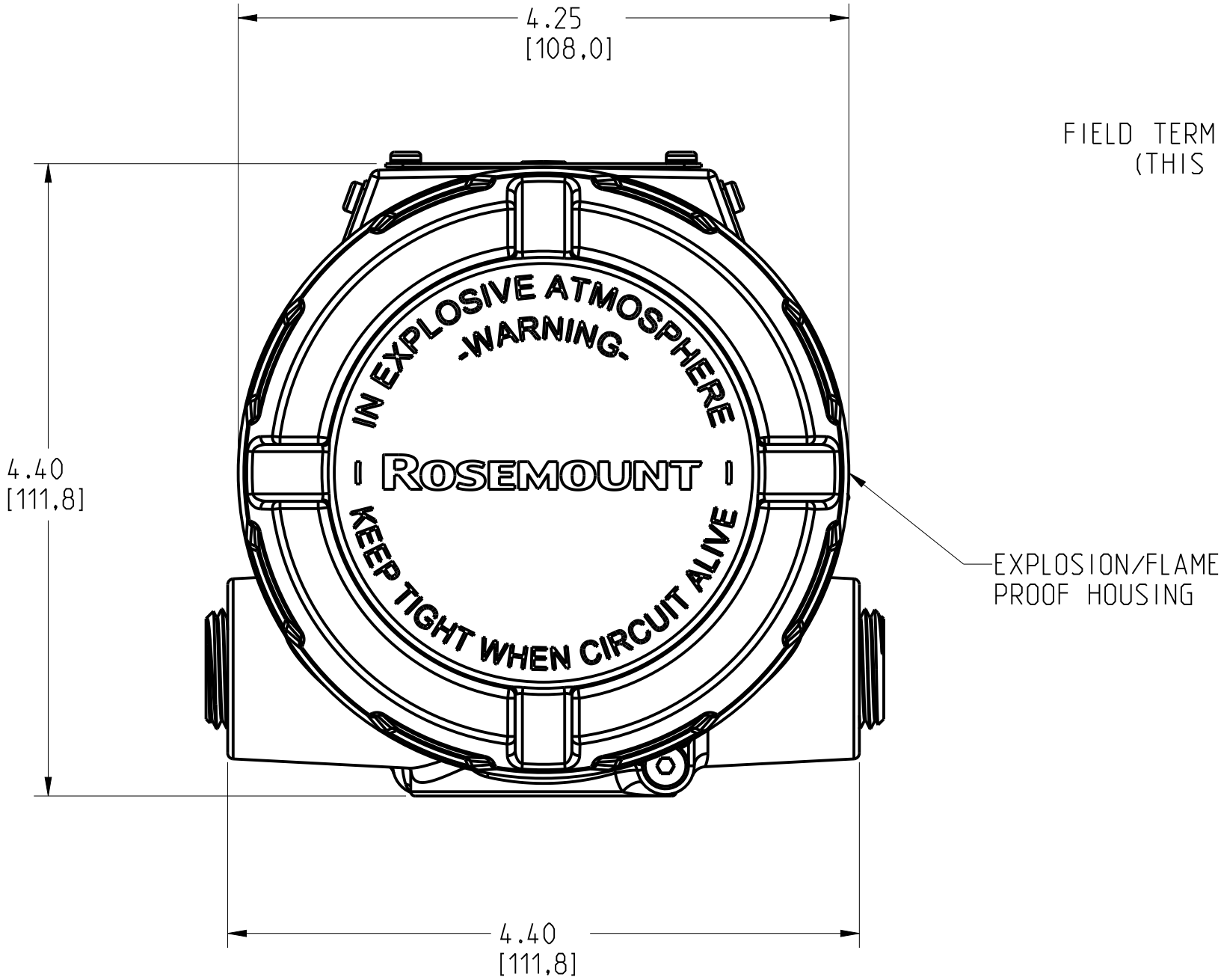
SHOWN WITH NO DIGITAL DISPLAY
