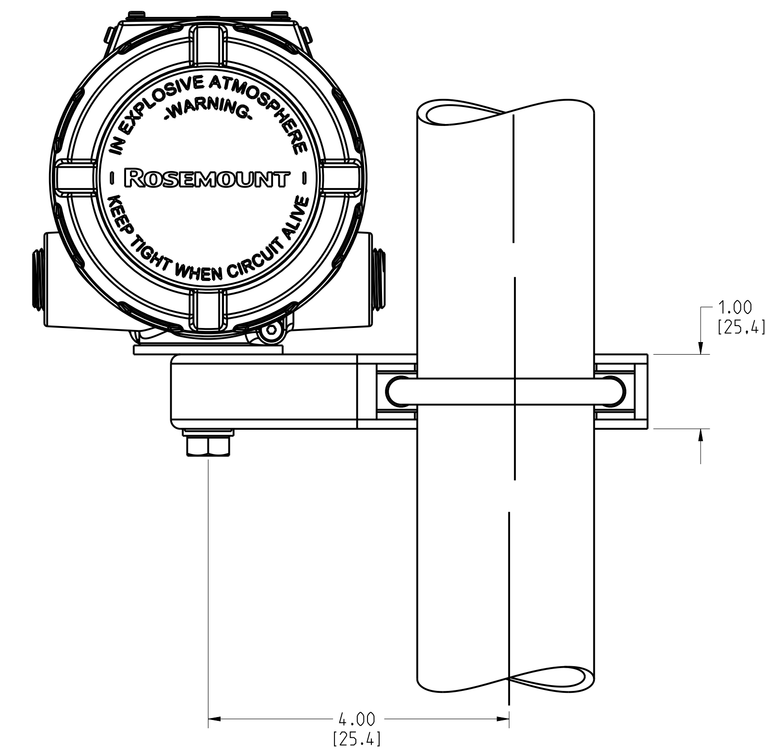
PIPE MOUNTING WITH L BRACKET OPTION (B5)
