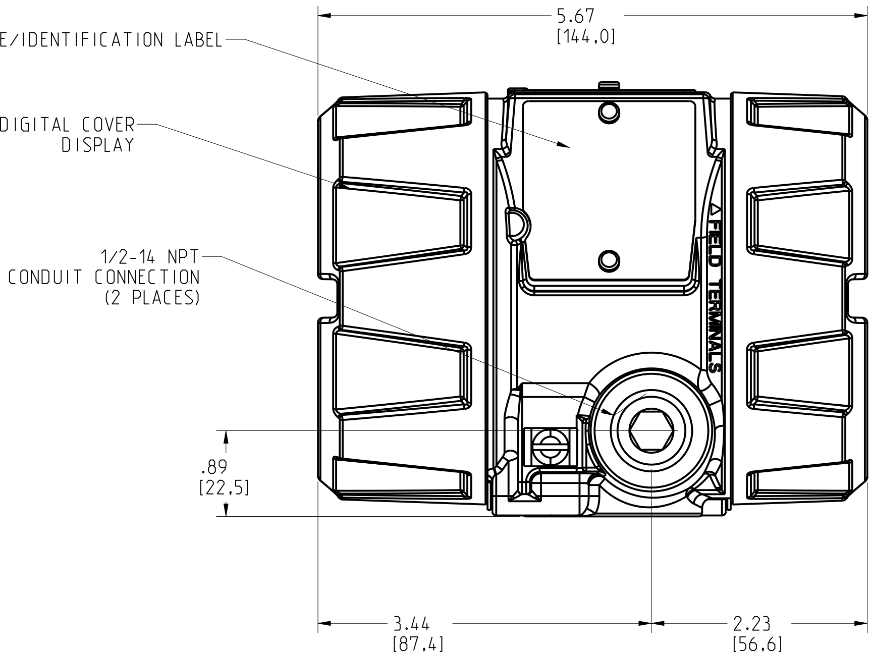
SHOWN WITH OPTIONAL DIGITAL DISPLAY
